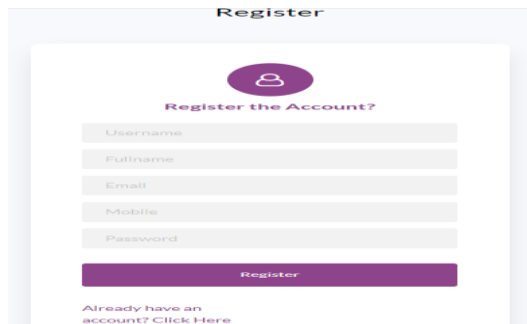
Fig 13 Registration page
