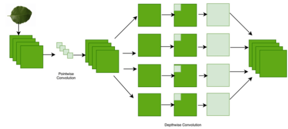
Fig 6 Xception architecture
