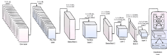
Fig 4 DenseNet169 architecture
