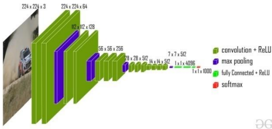
Fig 5 VGG16 architecture
