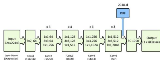
Fig 3 ResNet50 architecture
