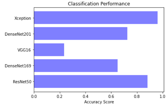
Fig 8 Accuracy Graph
