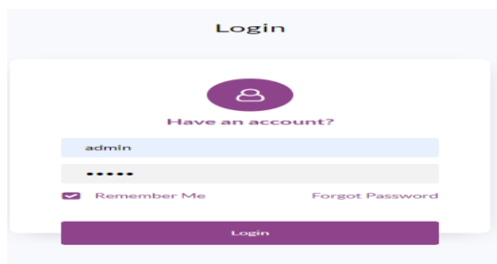
Fig 14 Login page
