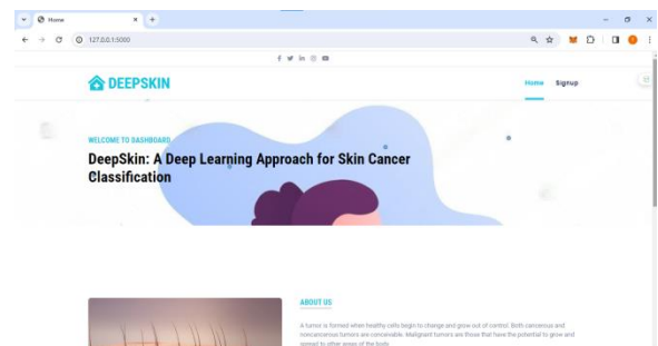
Fig 12 Home page
